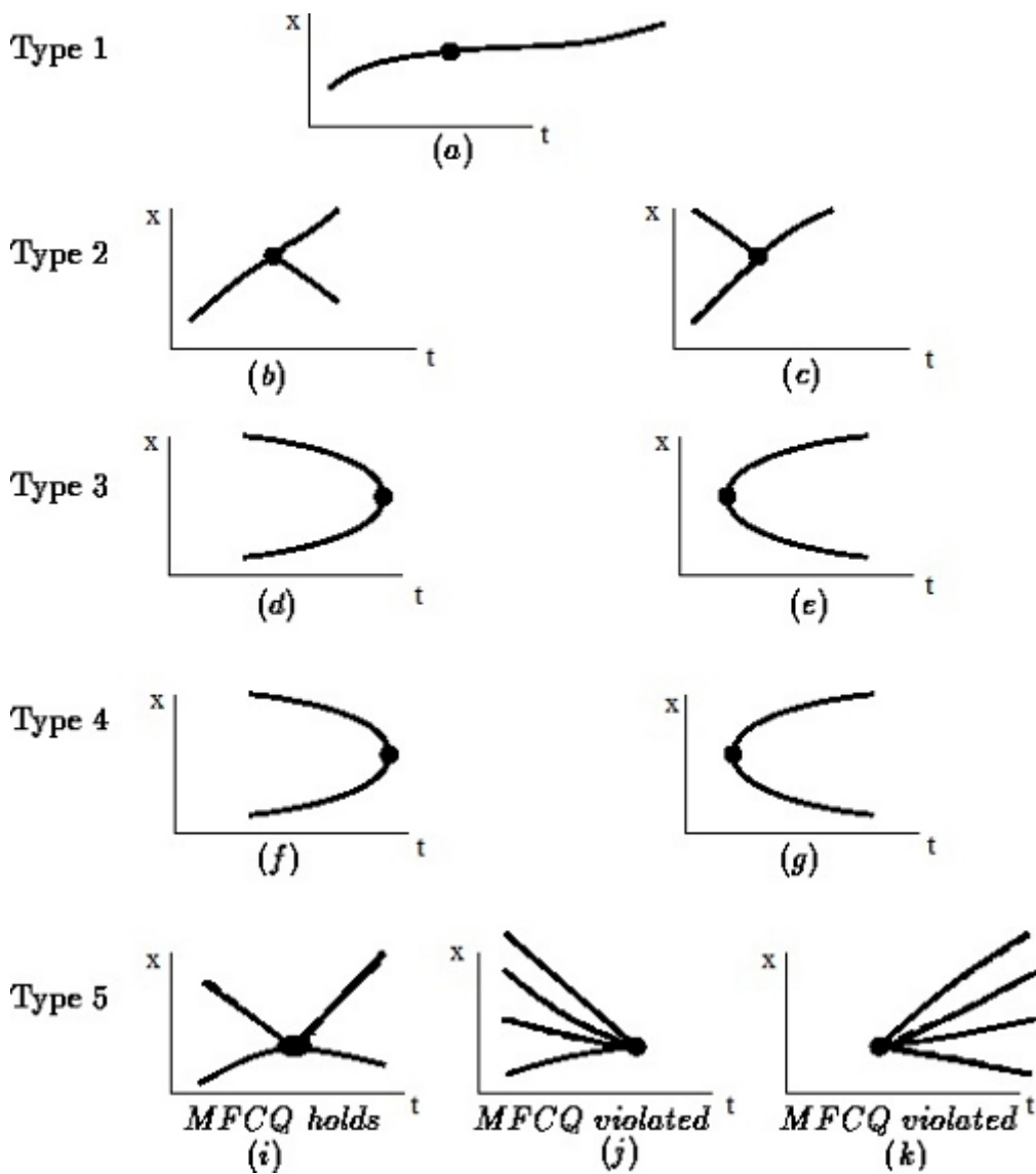
Fig. 1. Local structure of \Sigma_{gc} .
