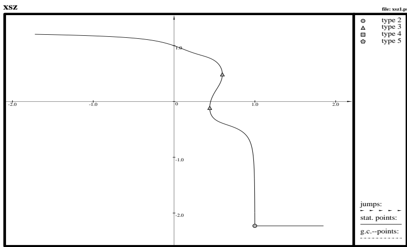
Fig. 3. x_1 vs. t .
