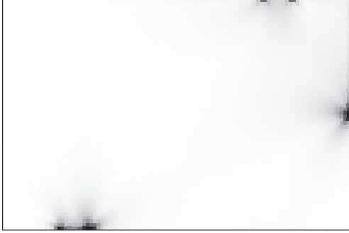
Figure 2: Primal error distribution
