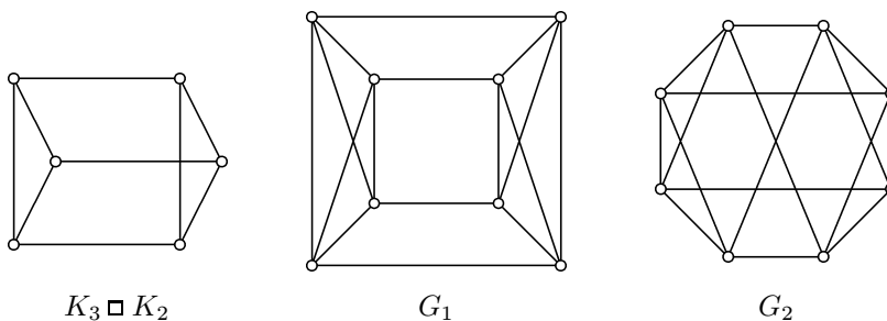
Figure 1. Regular Graphs Achieving Bound of Lemma 2.1.
