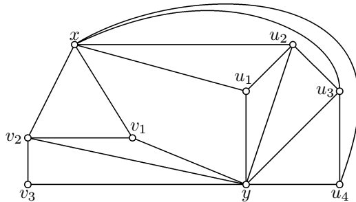
Figure 3. Planar Graph G such that d_c(G) = 2 .
