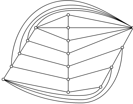
Figure 2. Planar Graph G such that d_c(G) = 3 .
