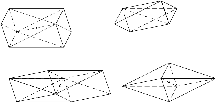
Figure 3. Examples of point-symmetric patches in three space dimensions.
