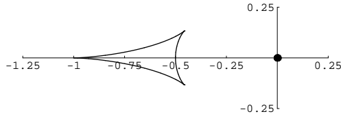
Figure 8. Curve of C5 type: a sextic reduced to one component with three cusps.
