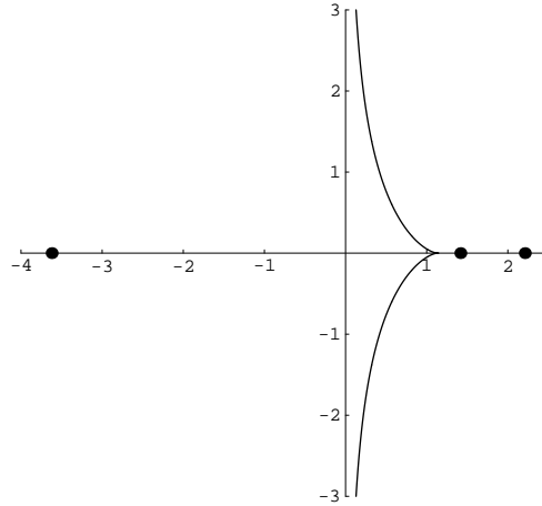
Figure 7. Curve of C4 type (Cissoid of Diocles) with a cusp in the real axis and a flex in the line of infinity. The imaginary axis is the flexional tangent and it corresponds to an asymptote of the curve.
