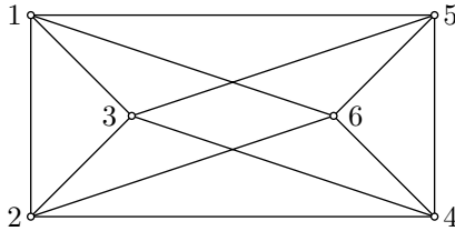
Figure 2. Graph with the (2, 2) -regular star set (co-star set) \{1, 3, 5\} for \mu = 0 .
