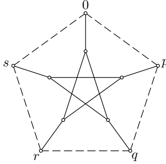
Figure 6. Graph with a (2,1) -regular star complement C_{6k-1} .
