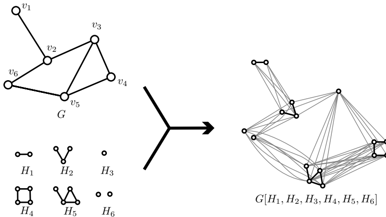
Figure 1. An example of graph cloning
