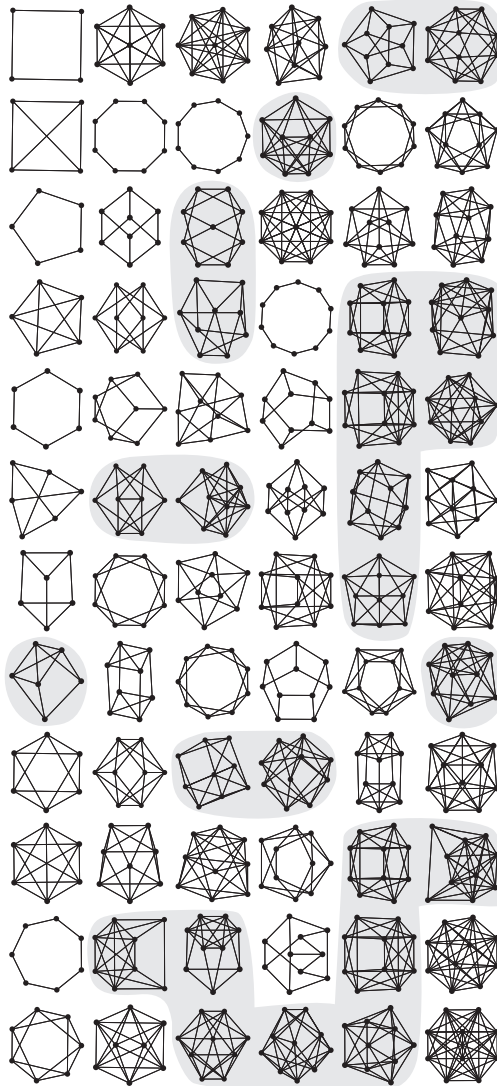
Figure 3: All betweenness-uniform graphs on 4–10 vertices (the grey graphs are not vertex transitive)
