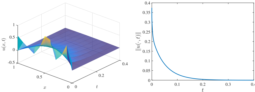
Fig. 3. State u(x,t) and norm \|u(\cdot, t)\| under control law (22), parameter update law (23) with \hat{\lambda}(0) = 0.1 , u_0(x) = rand(1) .
