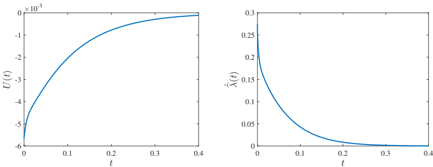
Fig. 4. Control law (22), parameter update law (23) with \hat{\lambda}(0) = 0.1 , u_0(x) = rand(1) .
