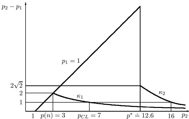
Figure 1. Functions \kappa_1, \kappa_2 for n = 2
