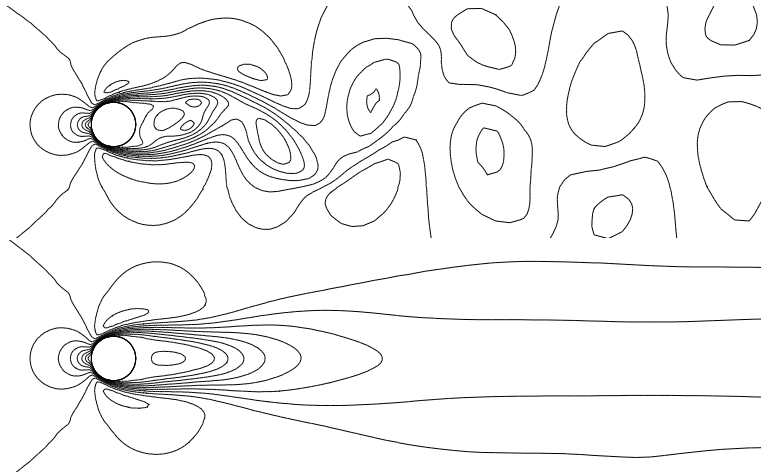
Figure 6: Isolines of velocity around cylinder in free space. Above: instantaneous velocity, below: time averaged velocity.
