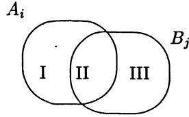
Fig. 3. Common and free elements of f -sets A_i and B_j .
