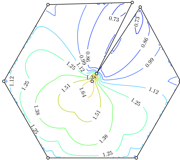
Figure 3. Contour plot of the quotient \delta_G(x, y)/\varrho_G(x, y) , when G is the polygon with vertices 1, e^{0.95\pi i/3}, 0.1e^{\pi i/3}, e^{1.05\pi i/3}, e^{2\pi i/3}, e^{\pi i}, e^{4\pi i/3}, e^{5\pi i/3} , the point x is fixed as 0, and y varies inside G .
