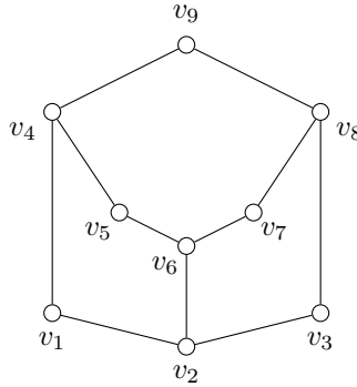
Figure 2. The unique extremal graph for R_1^\Delta(4, 6) = 10 .
