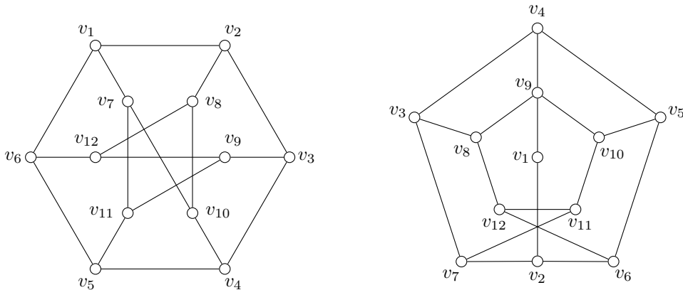
Figure 3. The two extremal graphs for R_1^\Delta(4, 7) = 13 .
