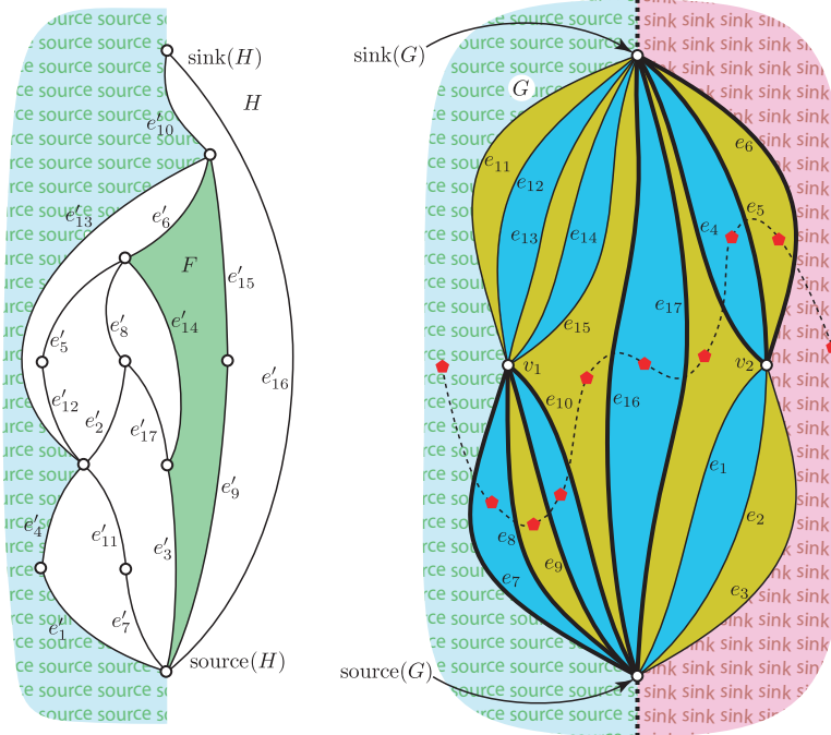
Figure 2. A facet F of H and the facets of G .
